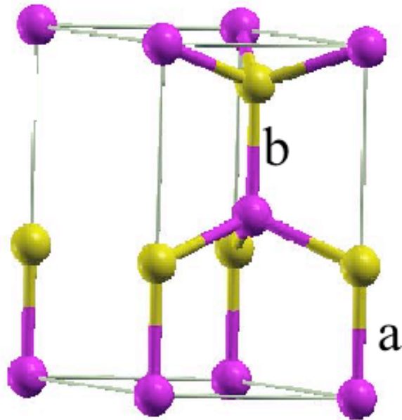
WZ along (0001)
