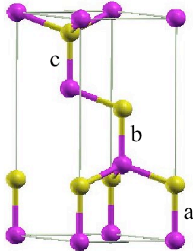
ZB along (111)
