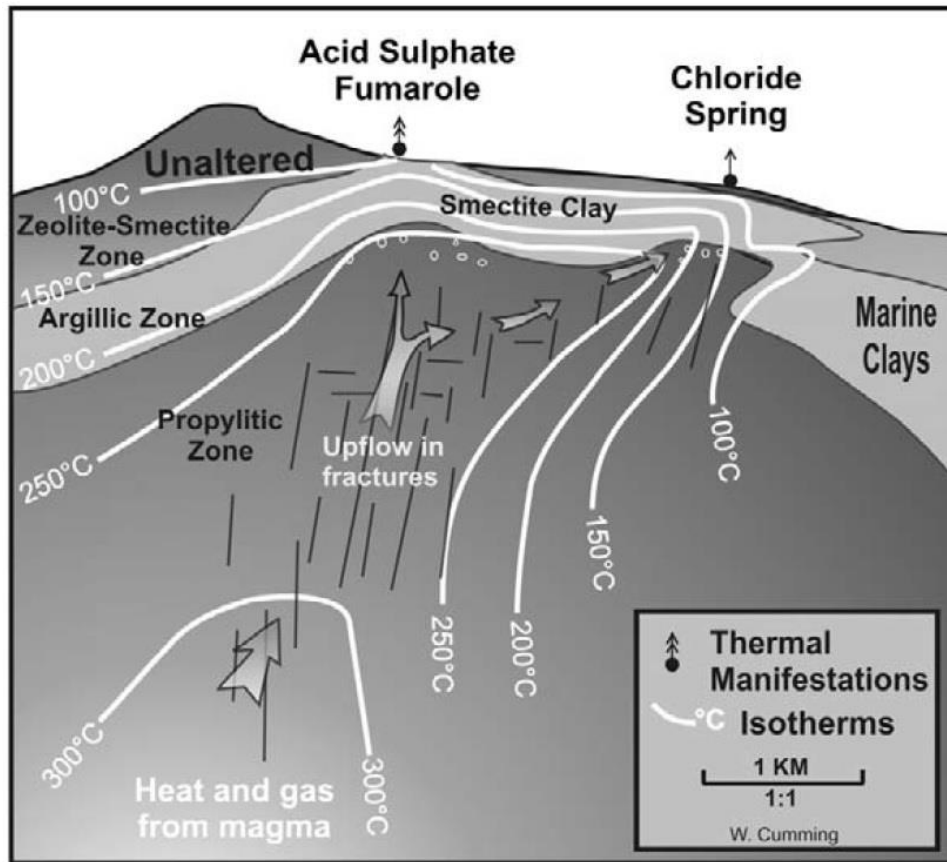
High-temperature system
