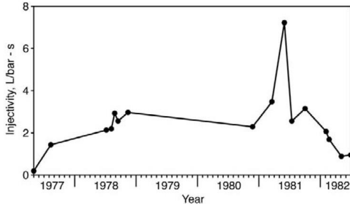
Injectivity history of well 4R1, Tongonan.
