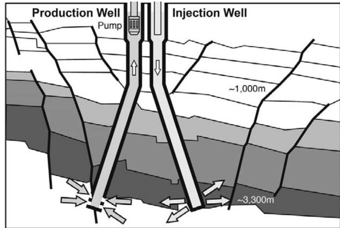
Low-temperature system
