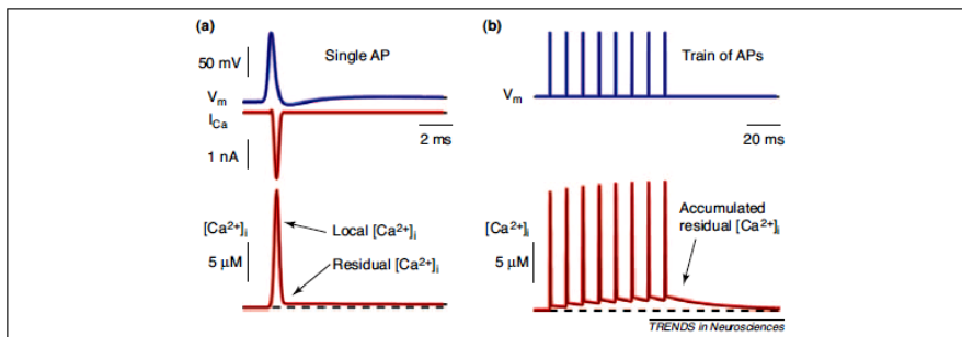
Figure 1. Schematic illustration of AP-evoked presynaptic [Ca 2+ ] i signaling at the release site. (a) A single AP (top panel) causes a short (~0.4 ms half-width) Ca 2+ current (I Ca ), which in turn creates a brief [Ca 2+ ] i transient at the release site ('local' [Ca 2+ ] i ). The local [Ca 2+ ] i signal is followed by a longer-lasting (i.e., ~30–50 ms) and widespread residual [Ca 2+ ] i signal of smaller amplitude (< ~0.5 μM). Residual [Ca 2+ ] i can cause a slower and asynchronous phase of release. (b) During a high-frequency train of APs (top panel), the residual [Ca 2+ ] i signal (bottom panel) can readily sum up to values in the low μM range, leading to increased rates of asynchronous release. Thus, phasic transmitter release during the presynaptic AP and the synchronous release phase are driven by local [Ca 2+ ] i signals with profoundly different amplitudes and kinetics.
