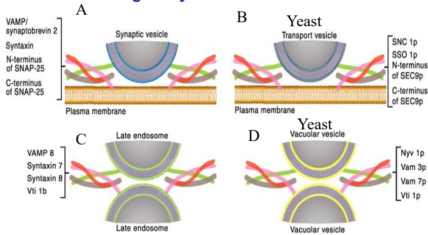
FIGURE 7 Neurotransmitter release shares a core mechanism with many membrane fusion events within eukaryotic cells. The fusion of synaptic vesicles (A) is driven by a particular complex of four coiled-coil domains contributed by three different proteins. Exocytosis in yeast (B), the fusion of late endosomes in mammalian cells (C), and the fusion of vacuolar vesicles in yeast (D) exemplify the closely related four-stranded coiled-coil complexes required to drive fusion in other membrane-trafficking steps.
