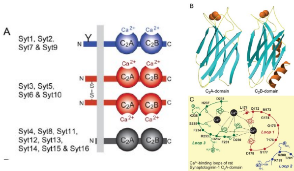
Figure 2. Structures and Ca^{2+} -binding properties of synaptotagmins. A. Canonical domain structures and classification of synaptotagmins. Mammals express 16 synaptotagmins composed of an N-terminal transmembrane region preceded by a short non-cytoplasmic sequence and followed by a variable linker sequence and two C2-domains; in addition, a 17 th related protein called B/K-protein contains the same domain structure but an N-terminal lipid anchor instead of the transmembrane region (see Pang and Südhof, 2010, for a discussion of additional synaptotagmin-related proteins). Eight synaptotagmins bind Ca^{2+} (Syt1, 2, 3, 5, 6, 7, 9, and 10; blue and red); the remaining synaptotagmins do not (black). The eight Ca^{2+} -binding synaptotagmins fall into two broad classes that differ in the absence (Syt1, 2, 7 and 9; blue) or presence (Syt3, 5, 6, and 10; red) of disulfide-bonded cysteine residues in their N-terminal sequences. Note that Syt1 and 2 include an N-glycosylated sequence at the N-terminus (indicated by a 'Y'), and that Syt7 is extensively alternatively spliced in the linker sequence (Han et al., 2004).
