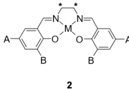
Figure 1. General structures for (1) chiral porphyrin and (2) chiral salen complexes.
