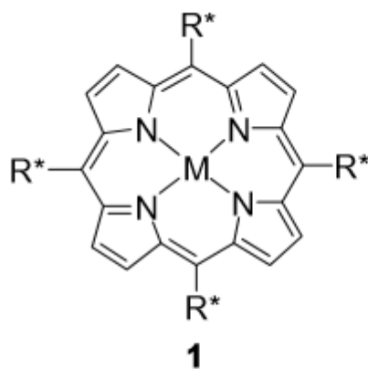
Figure 1. General structures for (1) chiral porphyrin and (2) chiral salen complexes.
