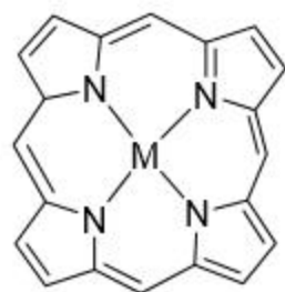
metalloporphyrin complex
