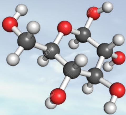
Glucosio
