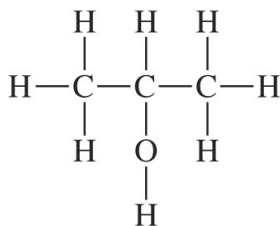
Dash formula
