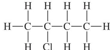
Dash formula
