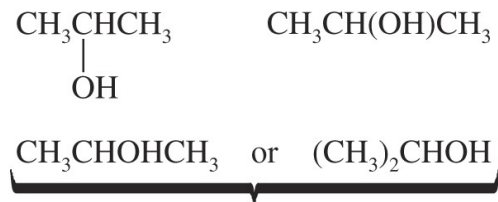
Condensed formulas
