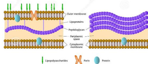
GRAM-NEGATIVE
