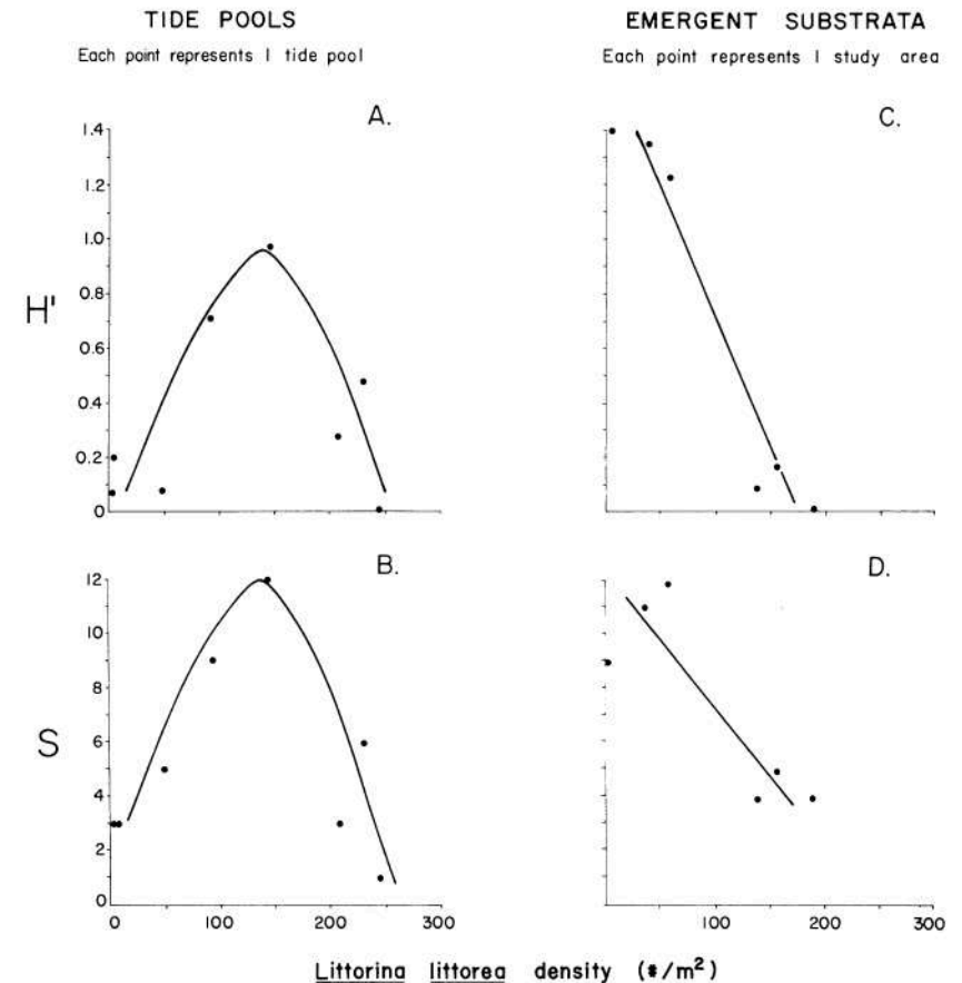
FIG. 3.—Effect of Littorina littorea density on the diversity of algae in high tide pools (A, B) and on emergent substrata in the low intertidal zone (C, D). S = no. species, H' is an index of diversity, here based on the percentage of cover of each species. Each point in A and B is from four (0.25 m 2 ) quadrats. Each point represents a different pool at Nahant, Massachusetts, September 1974. Each emergent substratum point was from 10 (0.25 m 2 ) quadrats in the low zone at six different areas in Massachusetts and Maine, June and July 1974 (see J. Menge [1975] for descriptions of areas). Regression equations: (A) tide pool H' = -0.0409 + 0.01250X - 0.00005X^2 , r^2 = .65 ; (B) tide pool S = 1.64 + 0.1357X - 0.00056X^2 , r^2 = .73 ; (C) low emergent substratum H' = 1.58 - 0.0089X , r^2 = .94 ; (D) low S = 11.58 - 0.0415X , r^2 = .72 . For mid-zone regressions (not illustrated), density of L. obtusata was converted to units of L. littorea density where 1 g wet weight L. obtusata is presumed to be equal to 1 g wet weight L. littorea . X, then, = "units of L. littorea ," i.e., actual density of that snail plus presumably equivalent units of L. obtusata . Mid H' = 1.65 - 0.004X , r^2 = .91 ; mid S = 8.03 - 0.017X , r^2 = .81 .
