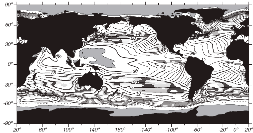
Average Sea-Surface Temperature for January
