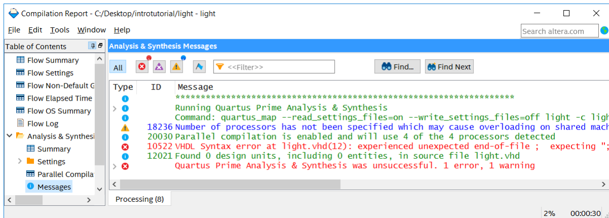
Figure 21. Error messages.
