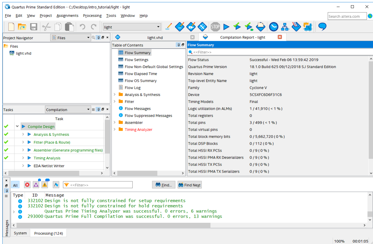
Figure 19. Display after a successful compilation.
