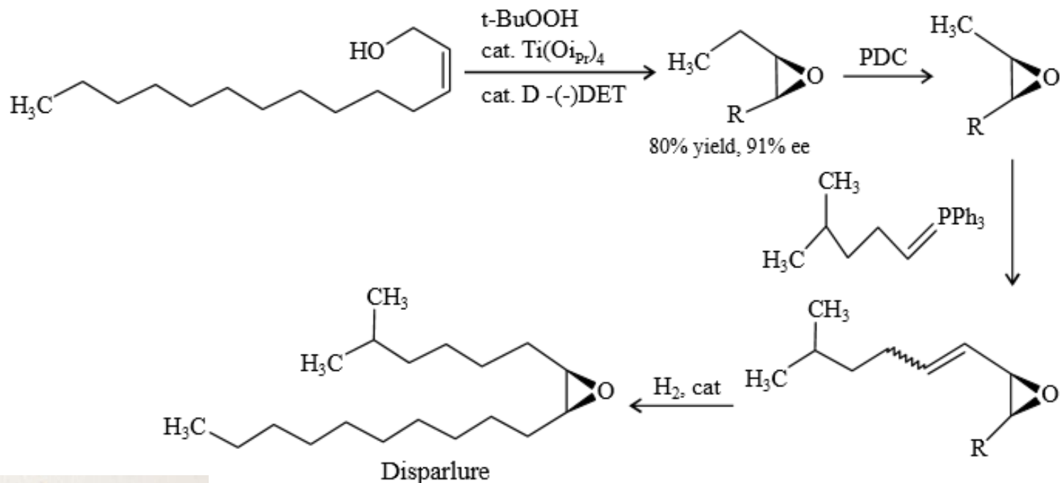
Scheme 17
