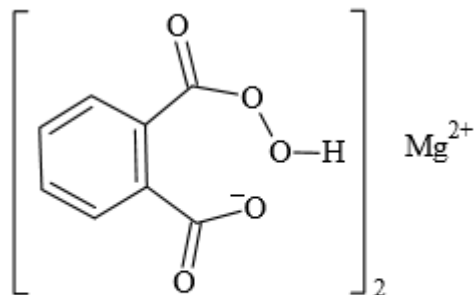
Magnesium monoperoxyphthalate (MMPBP)
