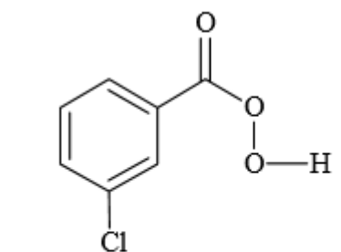
m-Chloroperoxybenzoic acid (MCPBA)
