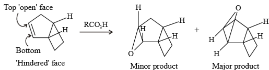
Scheme 5
