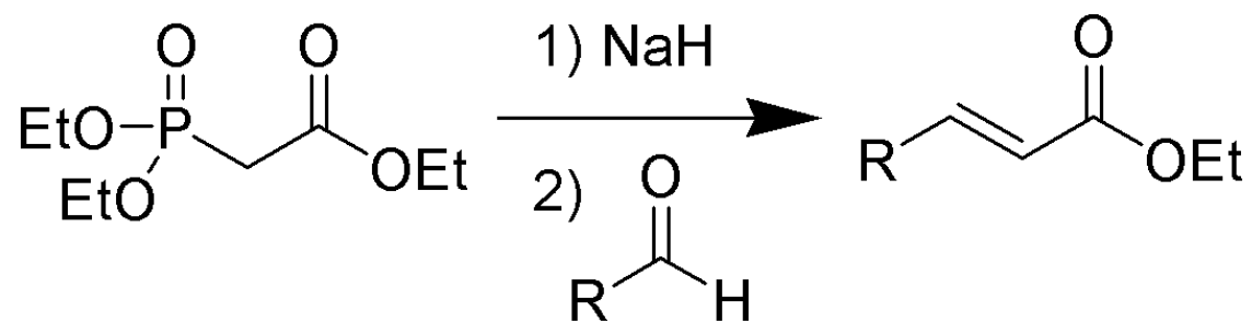
Horner-Wadsworth-Emmons
