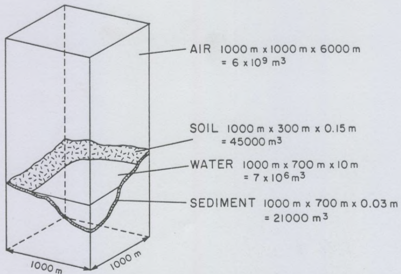
SIMPLE FOUR COMPARTMENT ENVIRONMENT
