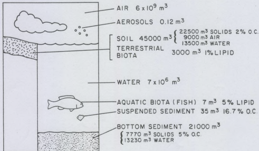
EIGHT COMPARTMENT ENVIRONMENT
