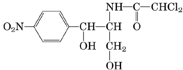
Chloramphenicol
