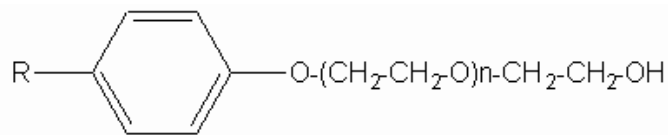
Alkylphenol polyethoxylate
