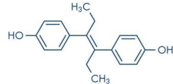
diethylstilbestrol
