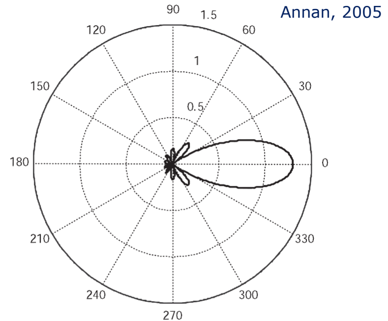
Figure 16. An example of antenna gain pattern. Similar plots can be created for directivity.
