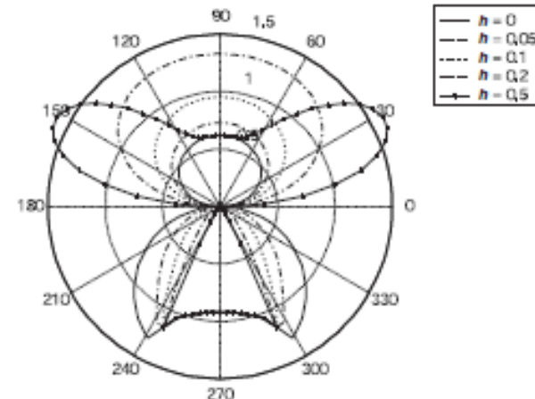
Figure 83. Antenna elevation also impacts directivity. The change in directivity is shown here as a function of height normalized against wavelength. MEMAG A.A. 2020-2021 8
