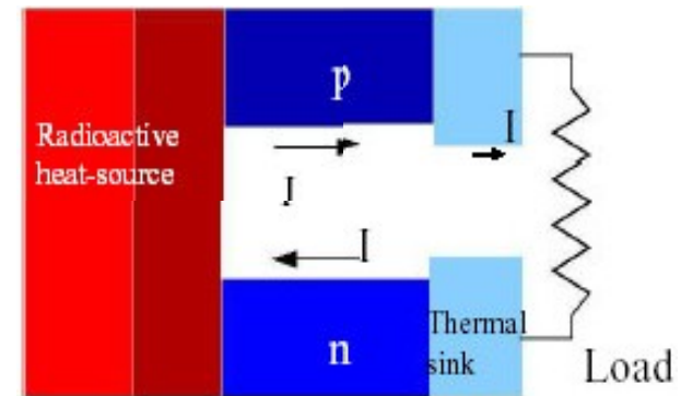
RTG Radioisotope Thermoelectric Generator Cassini-Huygens 1997
