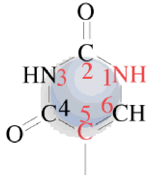
Pseudouridina ( \psi )
