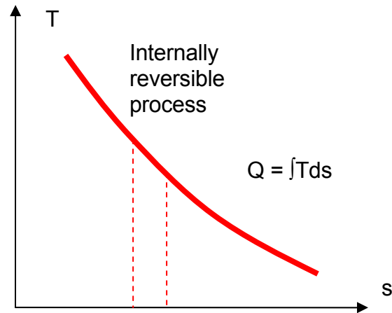
Fig. 6-2: On a T-s diagram, the area under an internally reversible process presents the heat transfer for the process.
