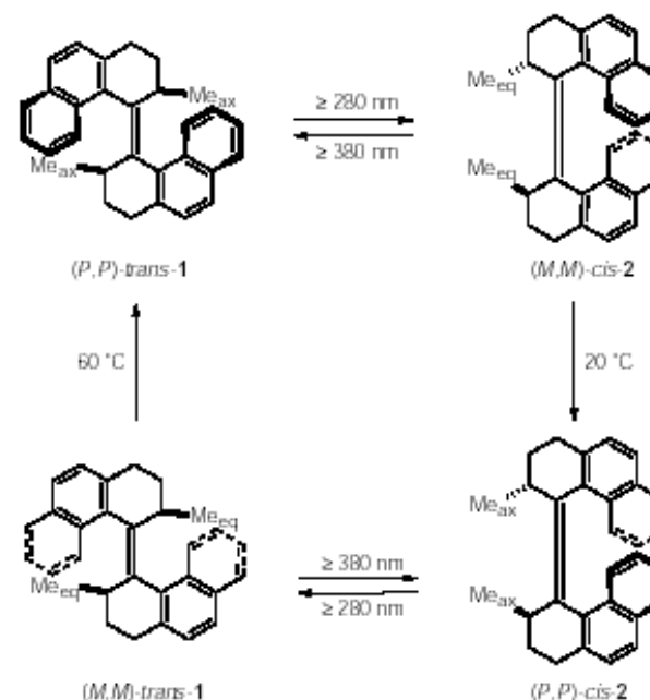
Figure 1 Photochemical and thermal isomerization processes of (P,P) - trans -1. UV irradiation with high pressure Hg-lamp, Pyrex filter, \lambda \geq 280 nm or Xe-lamp, Toshiba L-3g glass filter, \lambda \geq 380 nm. First order kinetics were observed for the thermal processes and temperature dependent ^1\text{H} NMR and CD studies in the range 50.0–81.1 °C gave E_a = 26.4 \text{ kcal mol}^{-1} for the (M,M) - trans -1 to (P,P) - trans -1 interconversion. It should be noted that no racemization takes place during any of the photochemical or thermal steps as was proven by chiral HPLC analysis of the isomers obtained after the individual steps.
