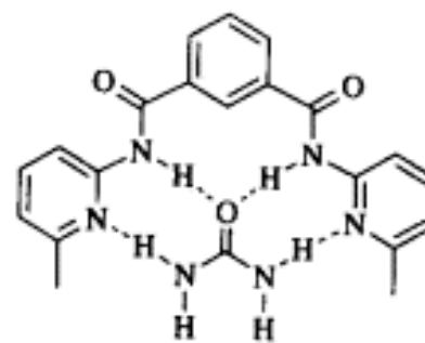
Urea Complex with 2
