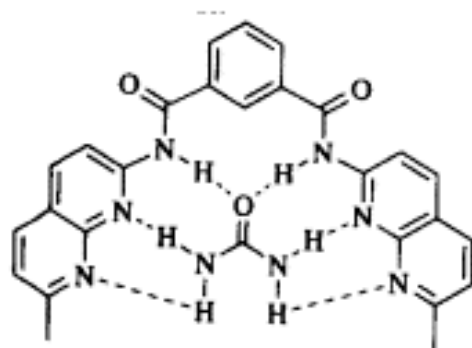
Urea Complex with 1
