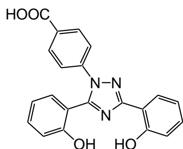
bis-hydroxyphenyl-triazole deferasirox
