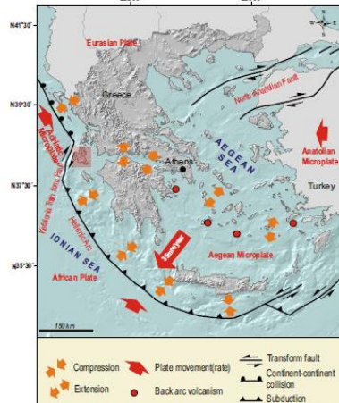
The geodynamic setting of the broader Aegean area
