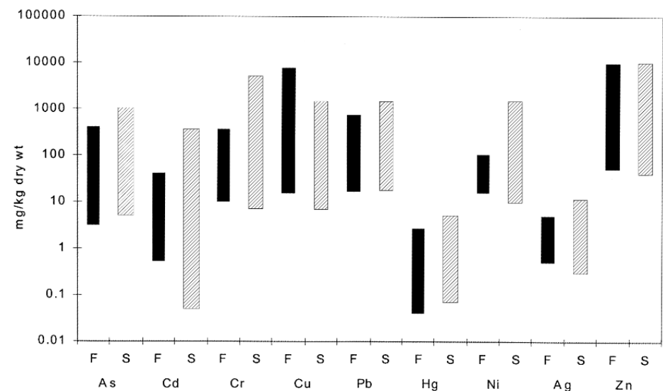
Fig. 1 Range of world-wide sediment quality values for selected metals and a metalloid (F=freshwater; S=saltwater). Not all values could be differentiated as indicating a concentration below which adverse effects were unlikely or, conversely, a concentration above which adverse effects were likely. Thus all values developed by any means, anywhere in the world, are shown.
