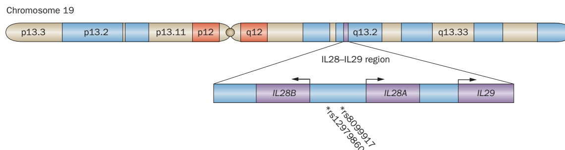
Figure 1 | The IL28–IL29 locus on chromosome 19. The genes encoding the three members of the IFN- \lambda family, IL28A (IFN- \lambda 2), IL28B (IFN- \lambda 3) and IL29, (IFN- \lambda 1) are clustered together on chromosome 19. The most important and validated SNPs with respect to response to IFN- \alpha therapy, rs12979860 and rs8099917, are upstream of both IL28B and IL28A (owing to their antiparallel orientation), but are physically closer to IL28B .
