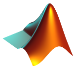
MATLAB logo
