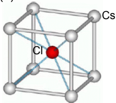
(a) CsCl
