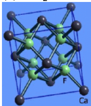
(c) CaF 2
