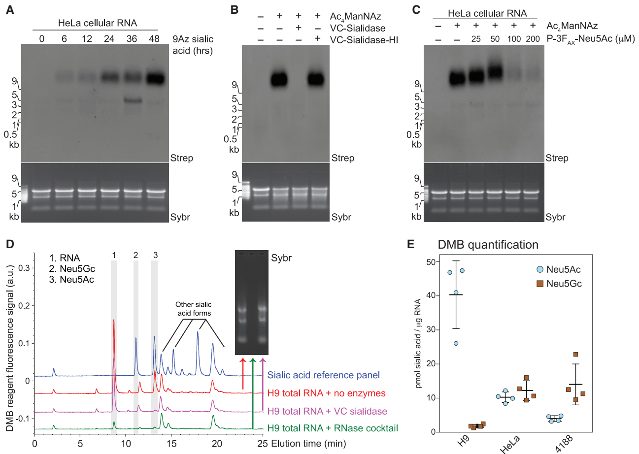
Figure 3. Glycans modifying RNA contain sialic acid
