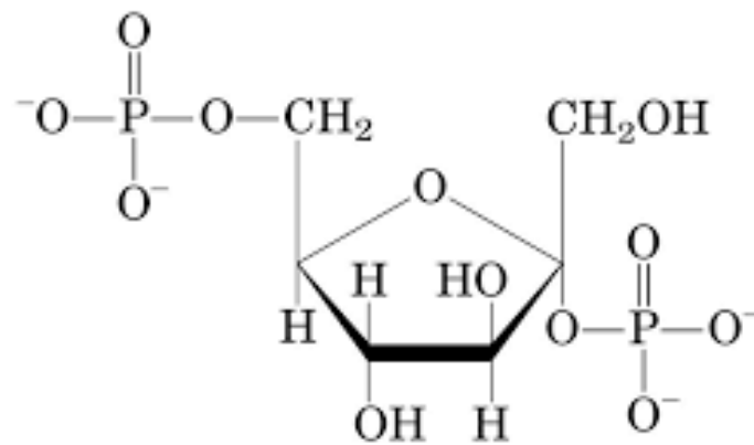
Fructose 2,6-bisphosphate
