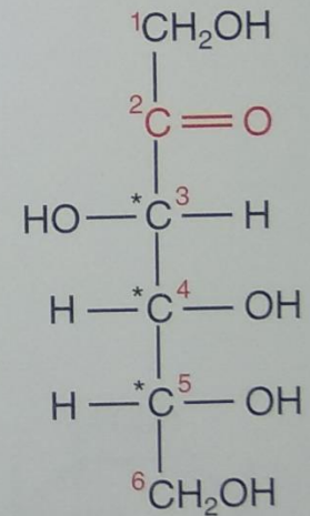
D-fruttosio
