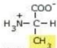
Alanina
