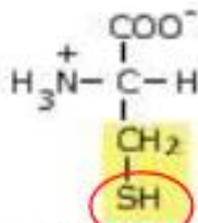
Cisteina
