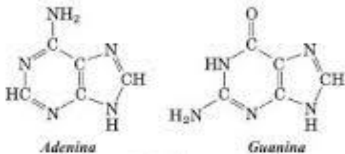
Purine
