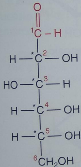
D-glucosio
