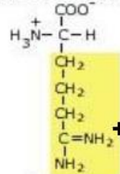
Arginina
