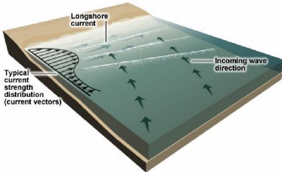
Longshore Current
