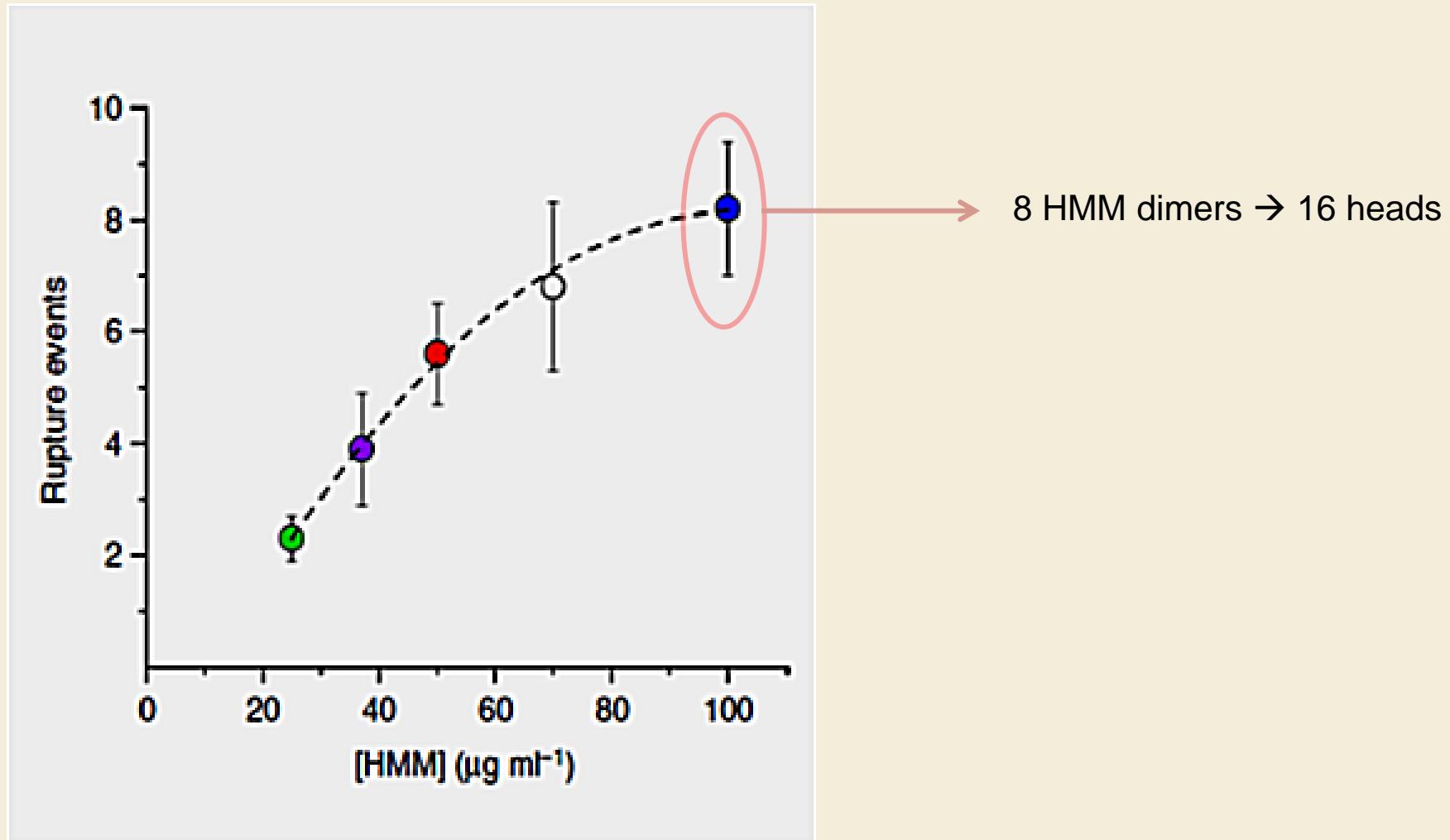
Number of rupture events vs HMM concentration
