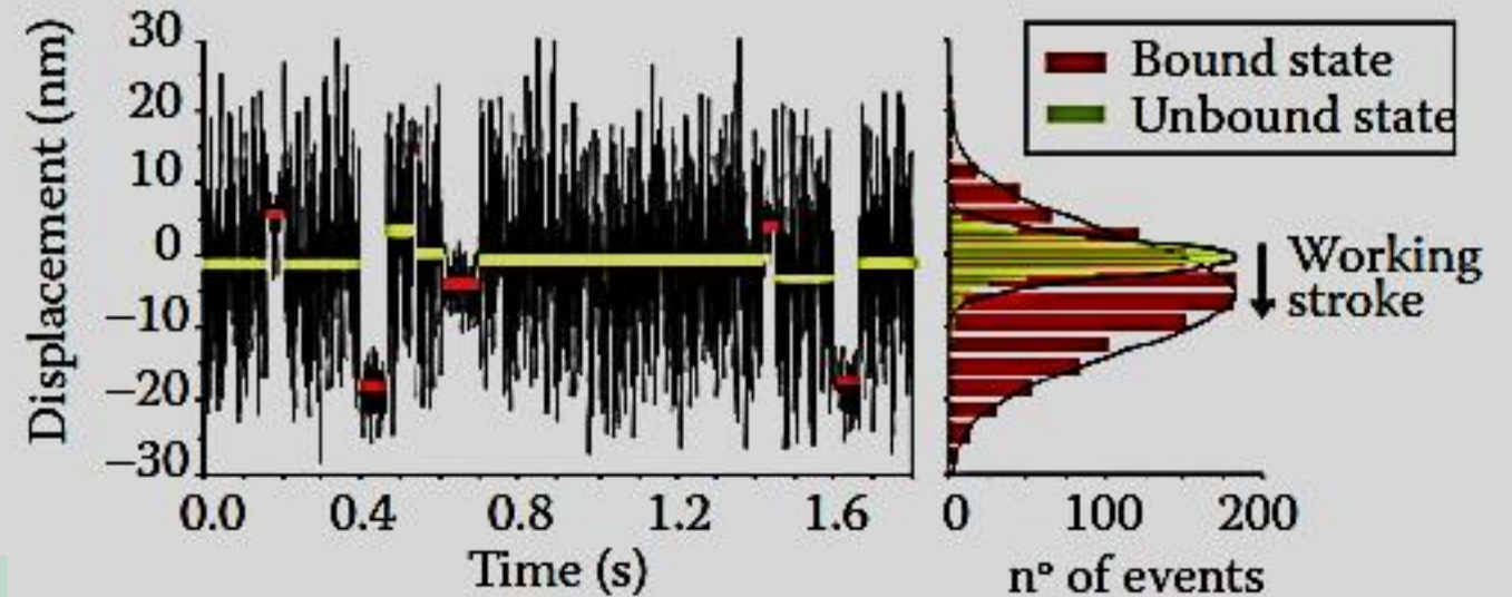
Position recording while myosin is interacting with actin.
