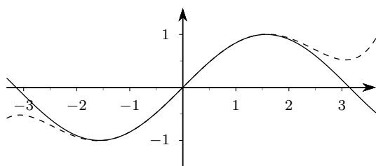
Figura 11.17 \sin x e T_{5,0}(x)
