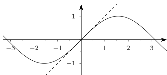
Figura 11.15 \sin x e T_{1,0}(x)
