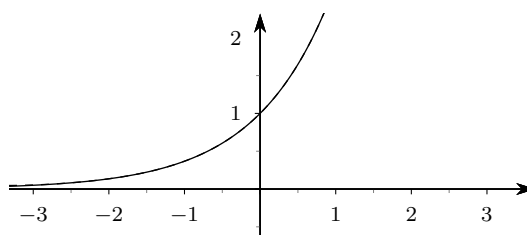
Figura 11.14 e^x e T_{10,0}(x)
