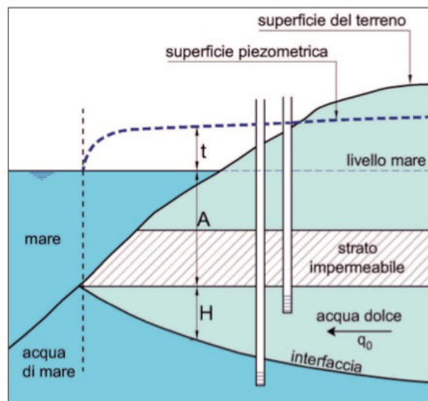
Fig. 5.11 - Intrusione marina in acquifero confinato costiero (mod., da VAN DAM, 1974). - Seawater intrusion in a confined coastal aquifer (modified from VAN DAM, 1974).
