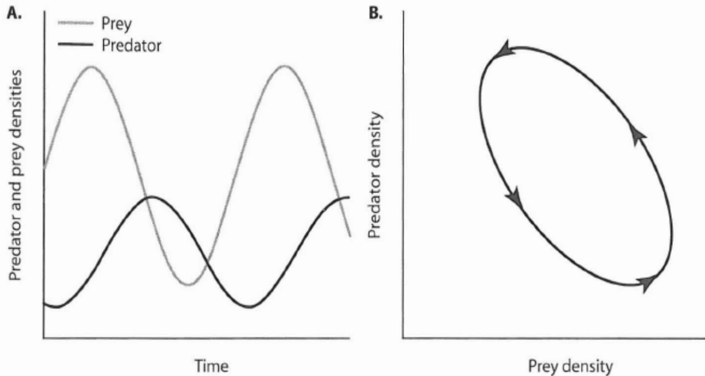
Figure 2. (A) Oscillating predator and prey populations and (B) a neutrally stable predator-prey limit cycle generated by the Lotka-Volterra equations.
