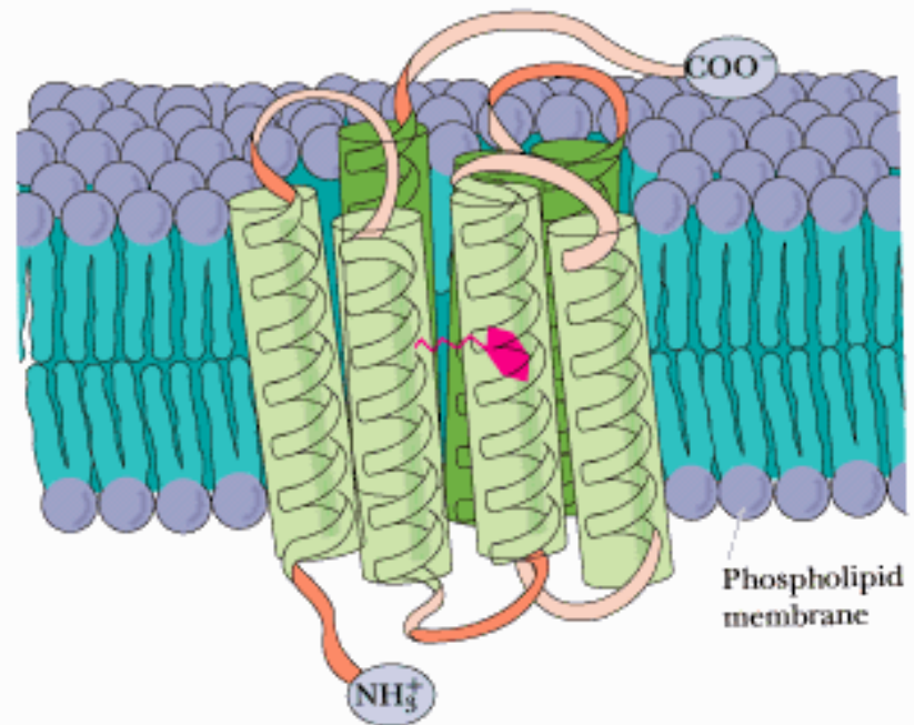
Bacteriorhodopsin
