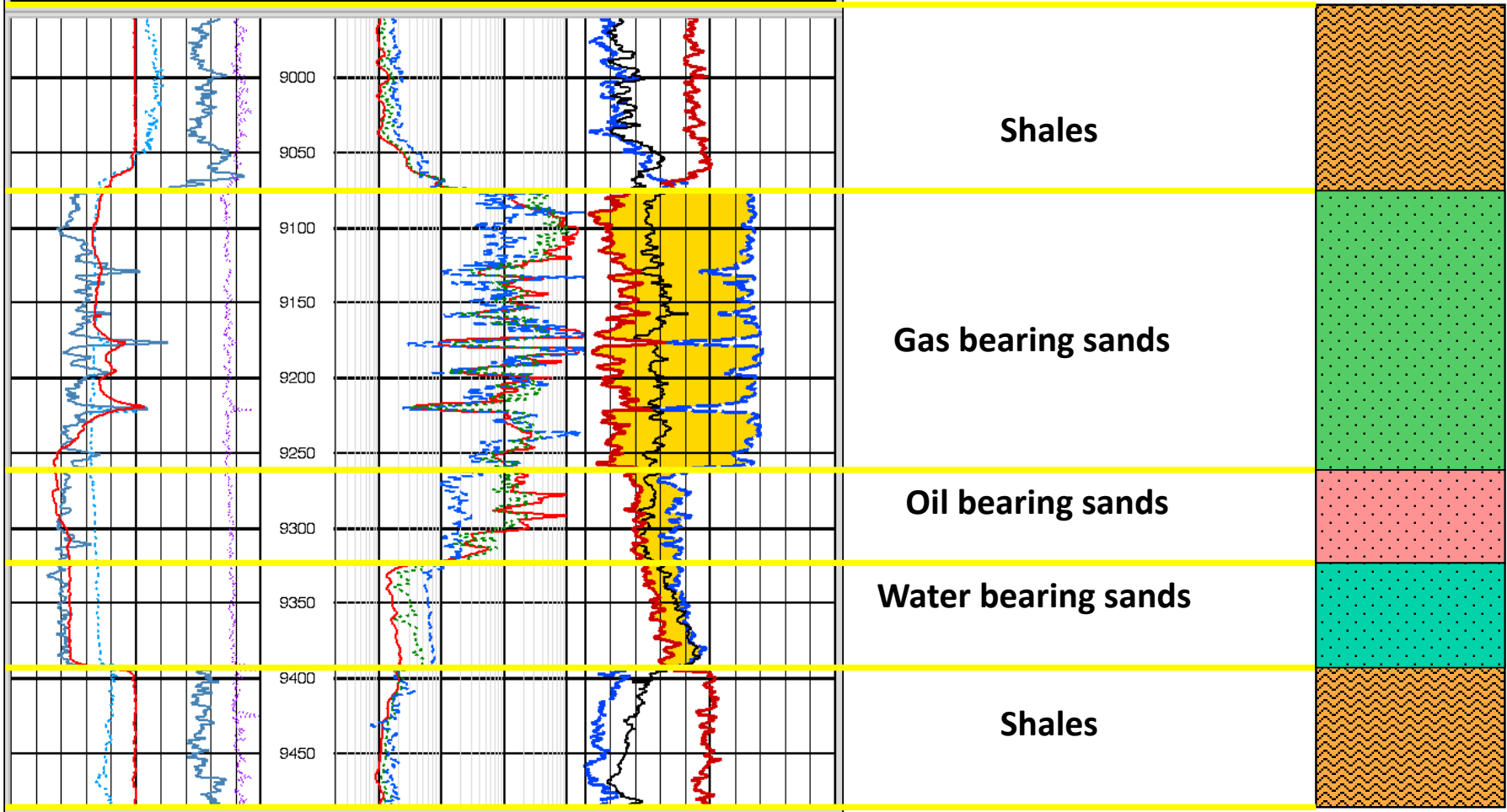
Basics of Geophysical well Logs_Porosity
