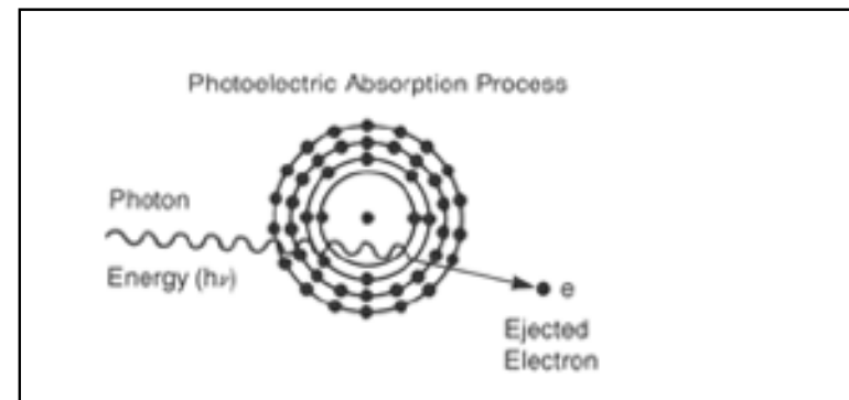
Photoelectric absorption process
