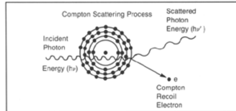
Compton scattering process
