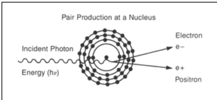
Pair production at a nucleus
