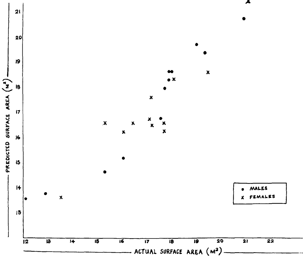
Figure 5. Plot of actual total surface area ( m^2 ) against predicted total surface area ( m^2 ) using the formula S = -8.245 + 6.807H + 7.073FFC in 24 adult Indian elephants irrespective of sex
