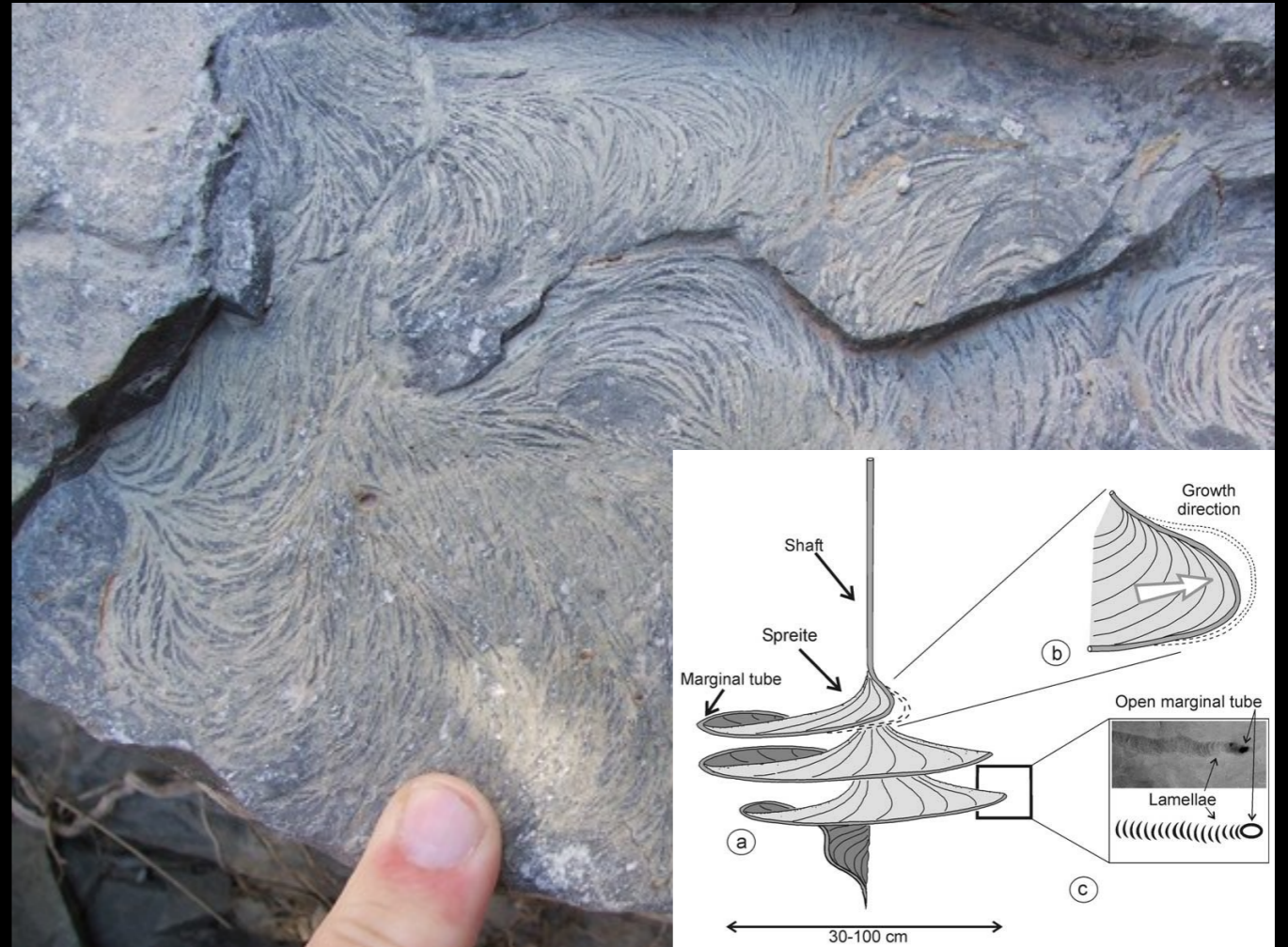
Zoophycos in Mississippian limestone from New Mexico (USA). Inset shows the shape and internal structure of a Zoophycos trace fossil.
