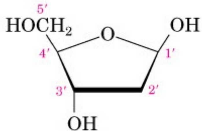
2'-Deossiribosio
