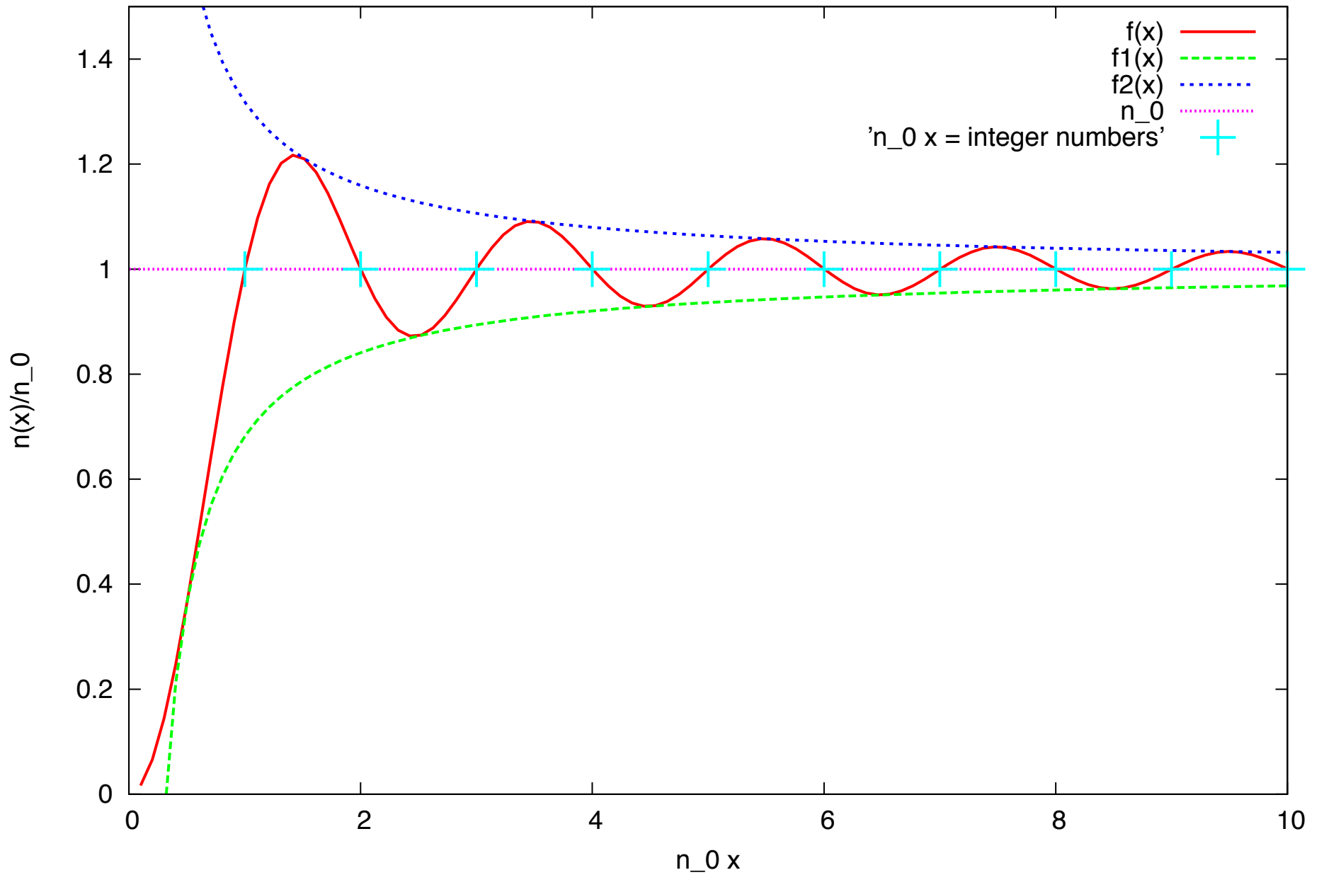
electron density in 1D with hard wall boundaries at x=0
