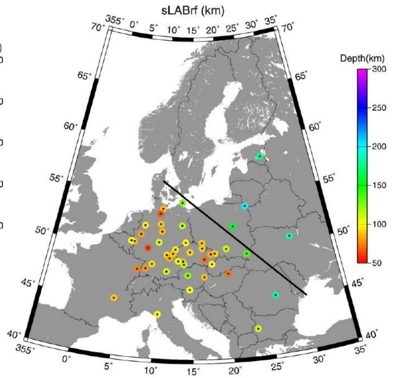
Seismic LAB (receiver functions)
