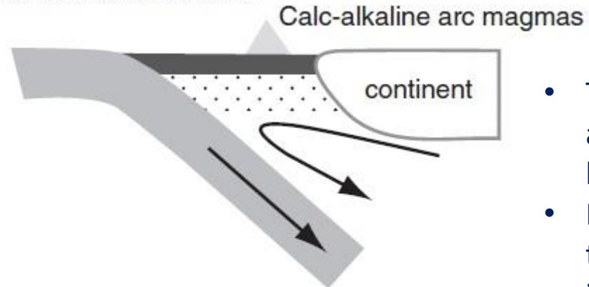
(b) Mature subduction zone
