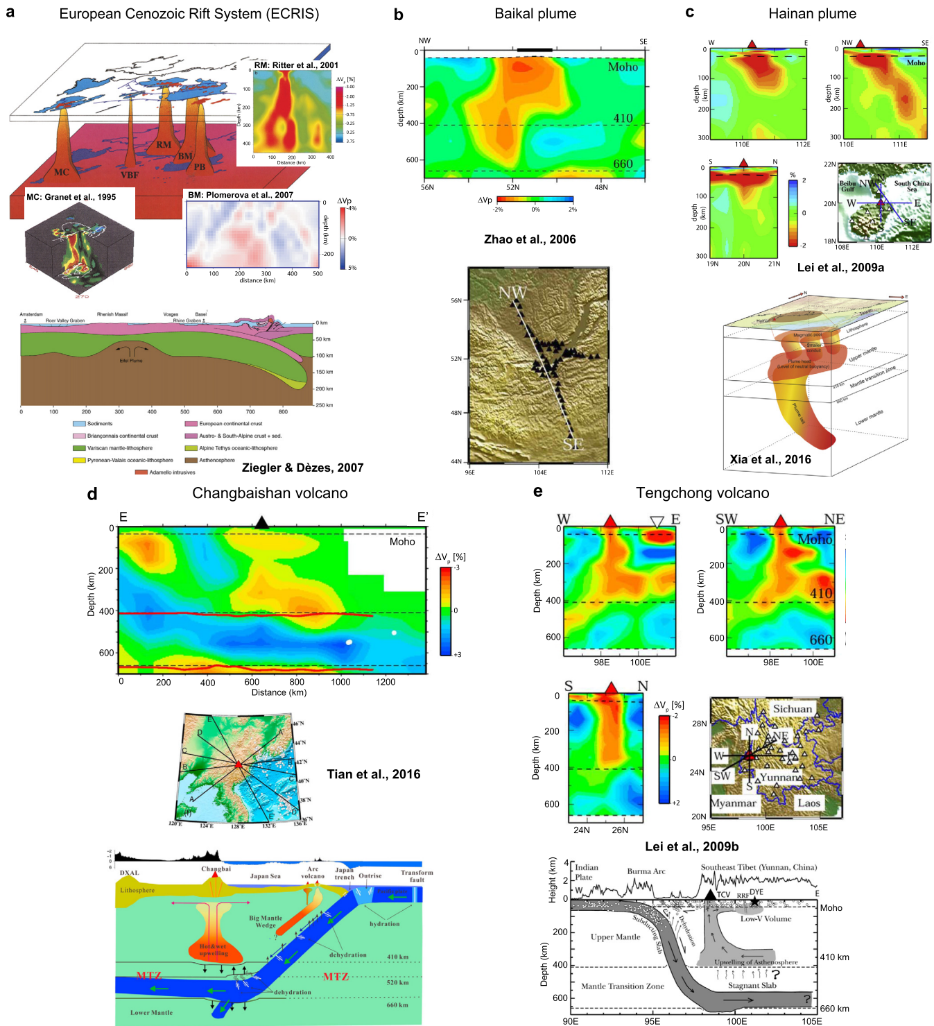
Fig. 2. Observations and conceptual interpretations of secondary plumes in different tectonic settings. a) European Cenozoic Rift System (ECRIS) plumes. Upper panel: Small-scale (baby) mantle plumes beneath different segments of the ECRIS (from Granet et al., 1995). Insets show seismic tomography images for the French Massif Central (from Granet et al., 1995), the Rhenish Massif/Eifel volcanic area (from Ritter et al., 2001), and the Bohemian Massif/Eger Graben (from Plomerová et al., 2007). Abbreviations: BM, Bohemian Massif; MC, Massif Central; PB, Pannonian Basin; RM, Rhenish Massif; VBF, Vosges-Black Forest. The areas marked in red and blue are Tertiary-Quaternary volcanic fields and Variscan basement massifs, respectively. Lower panel: Schematic lithospheric transect across the Central Alps and the Rhenish Massif showing the tectonic position of the Eifel plume developed within a continental foreland on the subducting plate (from Ziegler and Dèzes, 2007). b) Baikal plume. Upper panel: Tomographic image beneath the Baikal rift with negative P-velocity anomalies (up to 2%) extending down to the MTZ. Lower panel: Location of tomographic cross-section (from Zhao et al., 2006). c) Hainan plume. Upper panel: Structure of the Hainan plume in the upper mantle shown by three cross-sections of P-wave velocity perturbations (from Lei et al., 2009a). Lower panel: Interpreted whole-mantle structure of the Hainan plume. Apart from a large segment extending from the CMB in the lower mantle, several much smaller patches are imaged from the MTZ to the LAB (from Xia et al., 2016). d) Changbaishan volcano. Top panel: Vertical cross-section (profile E-E' in middle panel) of P-wave tomography through the Changbaishan volcano. Middle panel: Location of all acquired profiles. Bottom panel: Cartoon showing the main features of the structure and dynamics of the upper mantle beneath the Changbaishan volcano (from Tian et al., 2016). e) Tengchong volcano. Top and middle panels: Structure of the upper mantle in the Tengchong volcano area shown by three cross-sections of seismic tomography. Bottom panel: Schematic west-east vertical cross-section showing the upper mantle structure beneath the Indian plate, Burma Arc, and southeast Tibet (Yunnan, south-western China). Abbreviations: DYE, the 2003 Dayao earthquake zone; RRF, Red River fault; TCV, Tengchong volcano (from Lei et al., 2009b).
