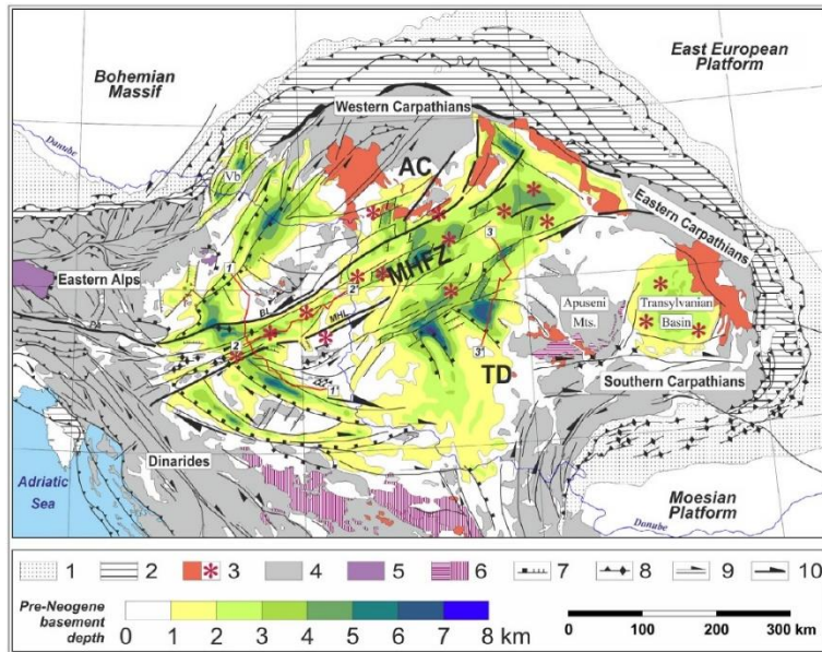
Crustal thinning
