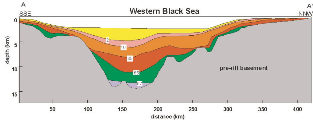
Observed WBS
