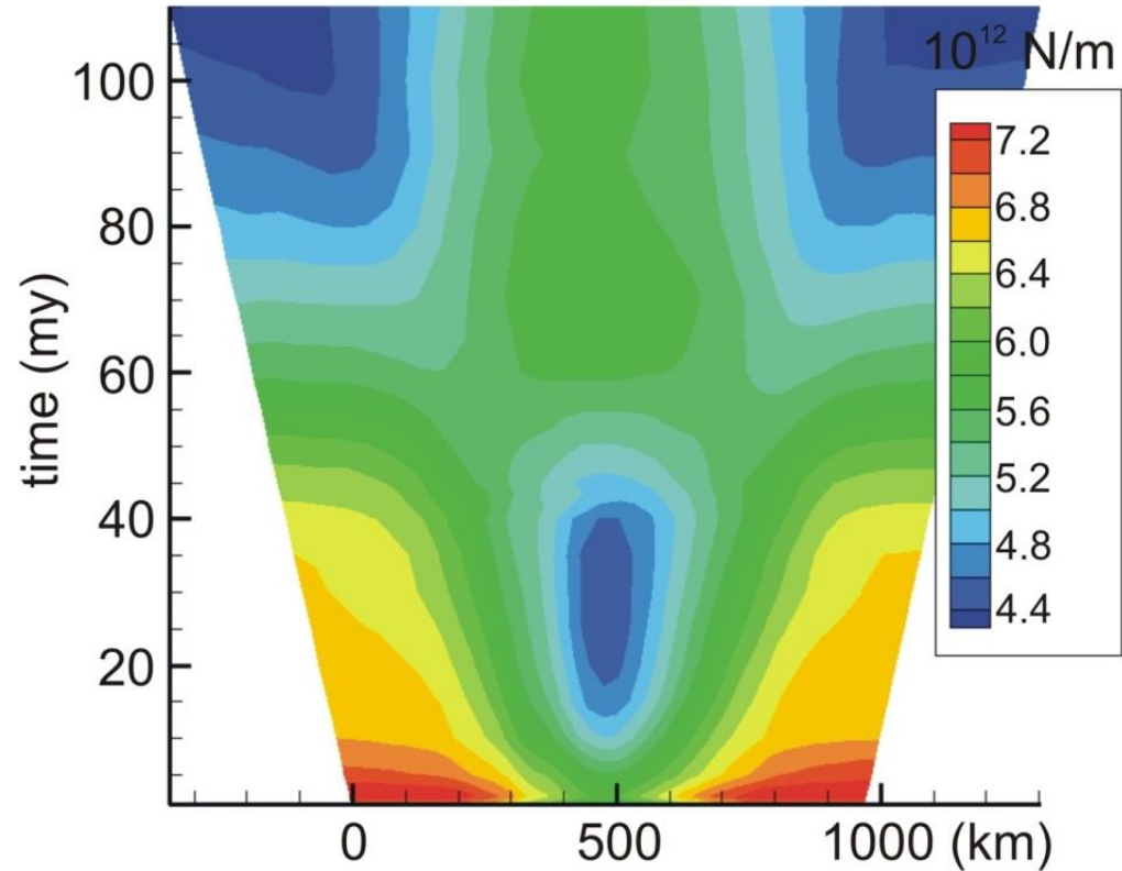
Slow extension
