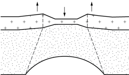
CONTINUOUS, DEPTH - DEPENDENT STRETCHING MODEL
