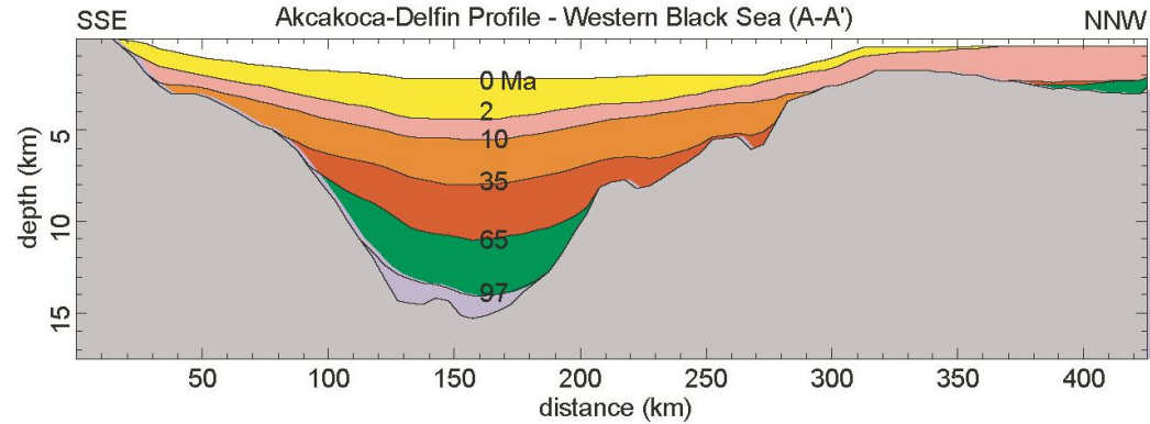
Predicted WBS
