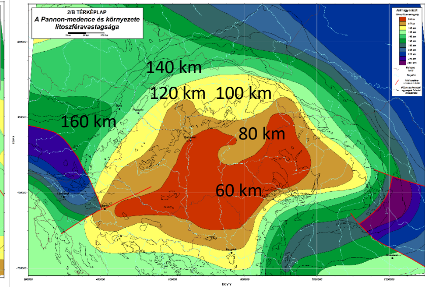
LAB
