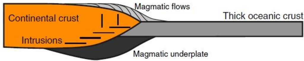
b Mode 2 excess-magmatic margins
