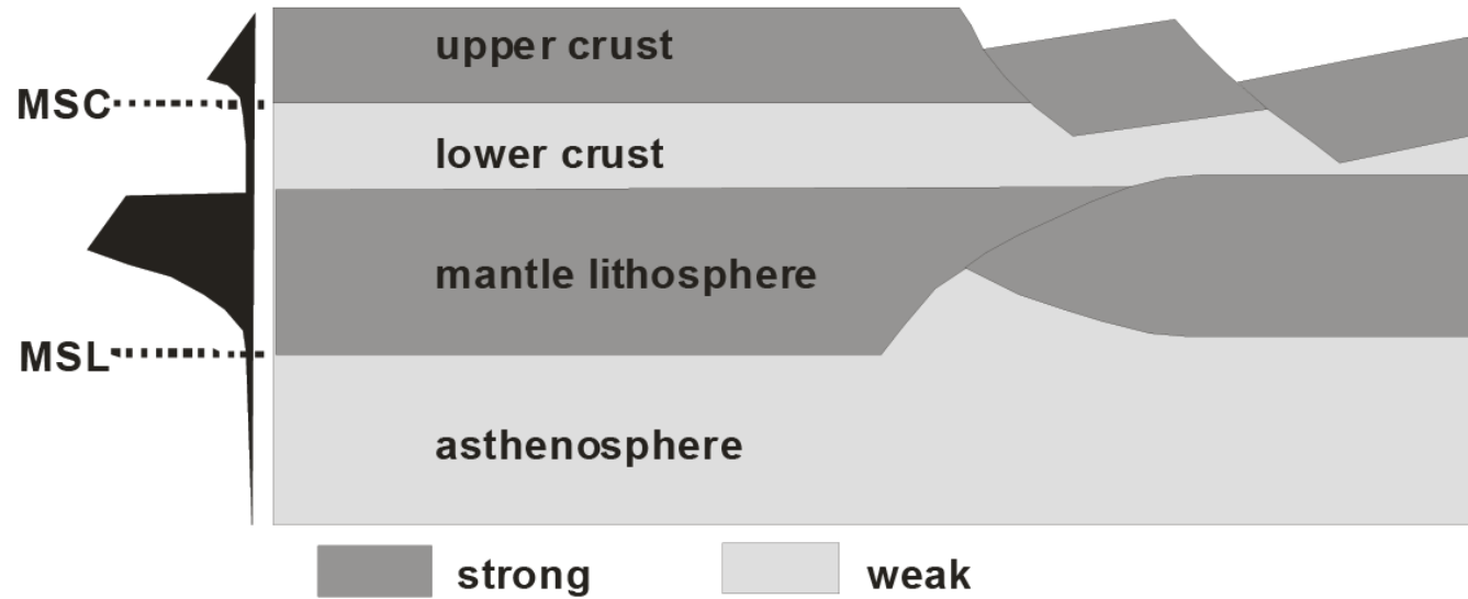
Kinematic model for extension of rheologically layered lithosphere
