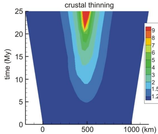
Fast extension (16 mm/yr)
