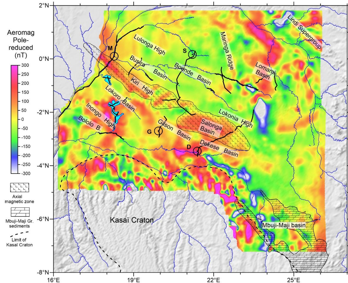
Aeromagnetic Anomalies
