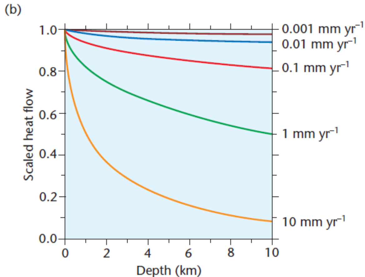
Basin thickness is the product of the sedimentation velocity and time
