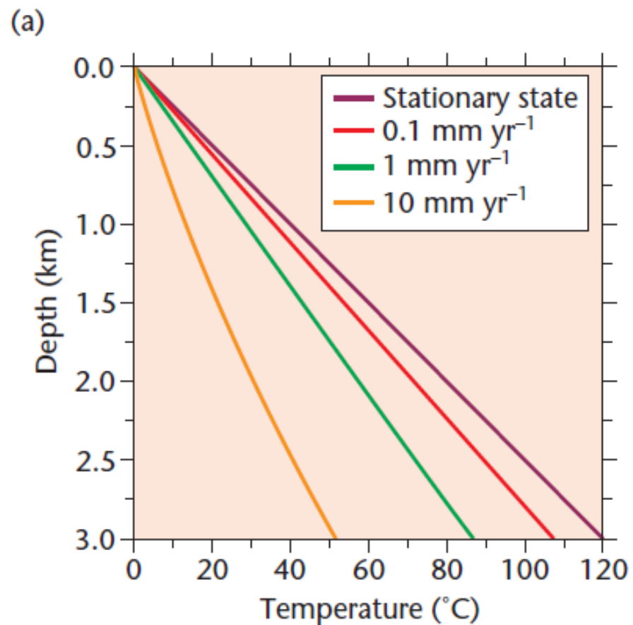
Geotherms at the time when 3 km of sediment has been deposited (30 Myr, 3 Myr and 0.3 Myr respectively).
