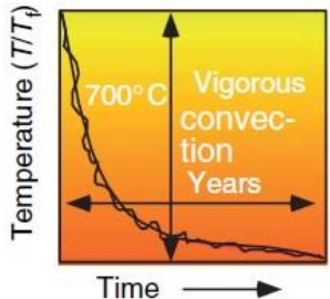
Sudbury impact melt sheet
