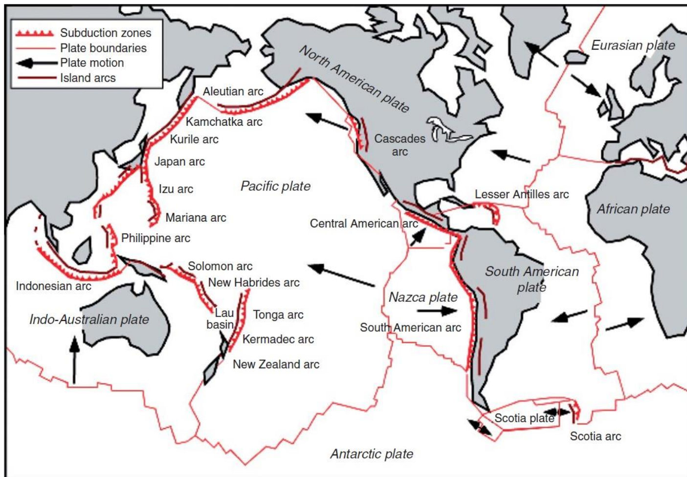
Marsh, 2007, Treatise of Geophysics, vol. 6
