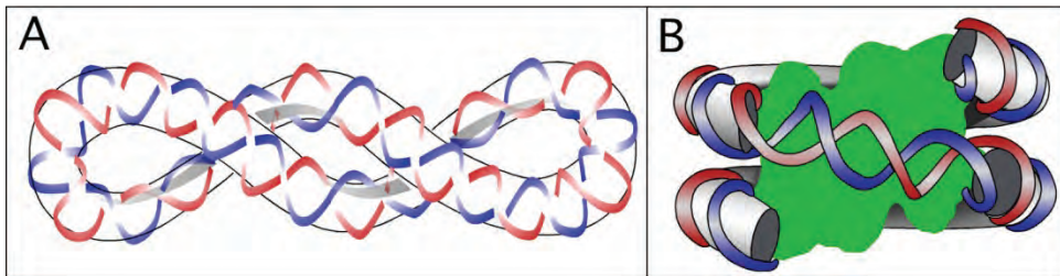
Fig. 7. Supercoiled DNA. A. Two negative supercoils are manifest as right-handed cross-overs in closed circular DNA. B. Similarly the DNA found in the nucleosome structure is wrapped \sim twice around the histone core proteins (green) to form two negative supercoils (adapted from (Luger, et al. , 1997)).
