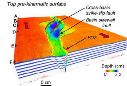
b 5° Transtension Model
