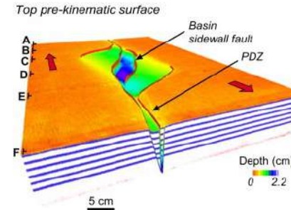
a Pure Strike-Slip Model
