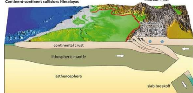
Continent-continent collision: Himalayas
