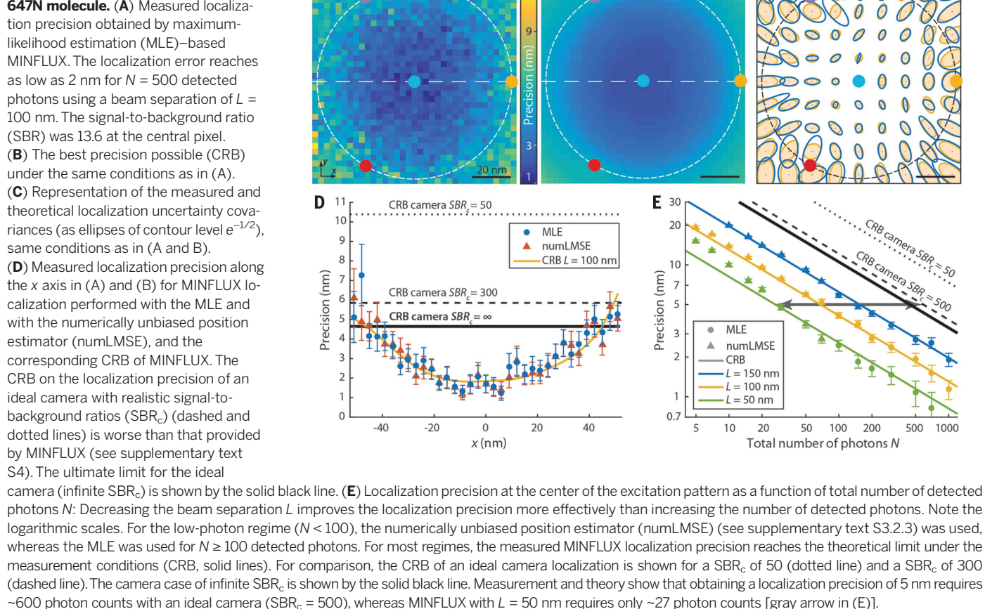
Fig. 3. Localization precision of MINFLUX measured on a single ATTO 647N molecule. (A) Measured localization precision obtained by maximum-likelihood estimation (MLE)-based MINFLUX. The localization error reaches as low as 2 nm for N = 500 detected photons using a beam separation of L = 100 nm. The signal-to-background ratio (SBR) was 13.6 at the central pixel. (B) The best precision possible (CRB) under the same conditions as in (A). (C) Representation of the measured and theoretical localization uncertainty covariances (as ellipses of contour level e^{-1/2} ), same conditions as in (A and B). (D) Measured localization precision along the x axis in (A) and (B) for MINFLUX localization performed with the MLE and with the numerically unbiased position estimator (numLMSE), and the corresponding CRB of MINFLUX. The CRB on the localization precision of an ideal camera with realistic signal-to-background ratios ( SBR_c ) (dashed and dotted lines) is worse than that provided by MINFLUX (see supplementary text S4). The ultimate limit for the ideal
