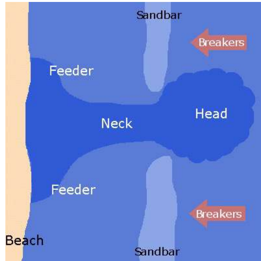
Rip Current Process: Cuspate Beach
