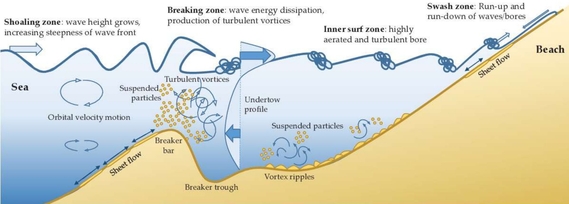
Figure 1.2. Conceptual drawing of cross-shore sediment processes in the near-shore region.
