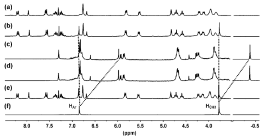
Figure 6. Partial ^1\text{H} NMR spectra (400 MHz, \text{CDCl}_3 ) of a) host 3 b) addition of 1 equiv of 1,4-( \text{MeO} ) _2\text{C}_6\text{H}_4 into host 3 solution without irradiation, c) 4 \odot 1,4-( \text{MeO} ) _2\text{C}_6\text{H}_4 , [16] d) c after 4 weeks in dark and RT, e) irradiation of c with light at 254 nm for 1 h or heating at 60°C for 20 min, f) guest 1,4-( \text{MeO} ) _2\text{C}_6\text{H}_4 .
