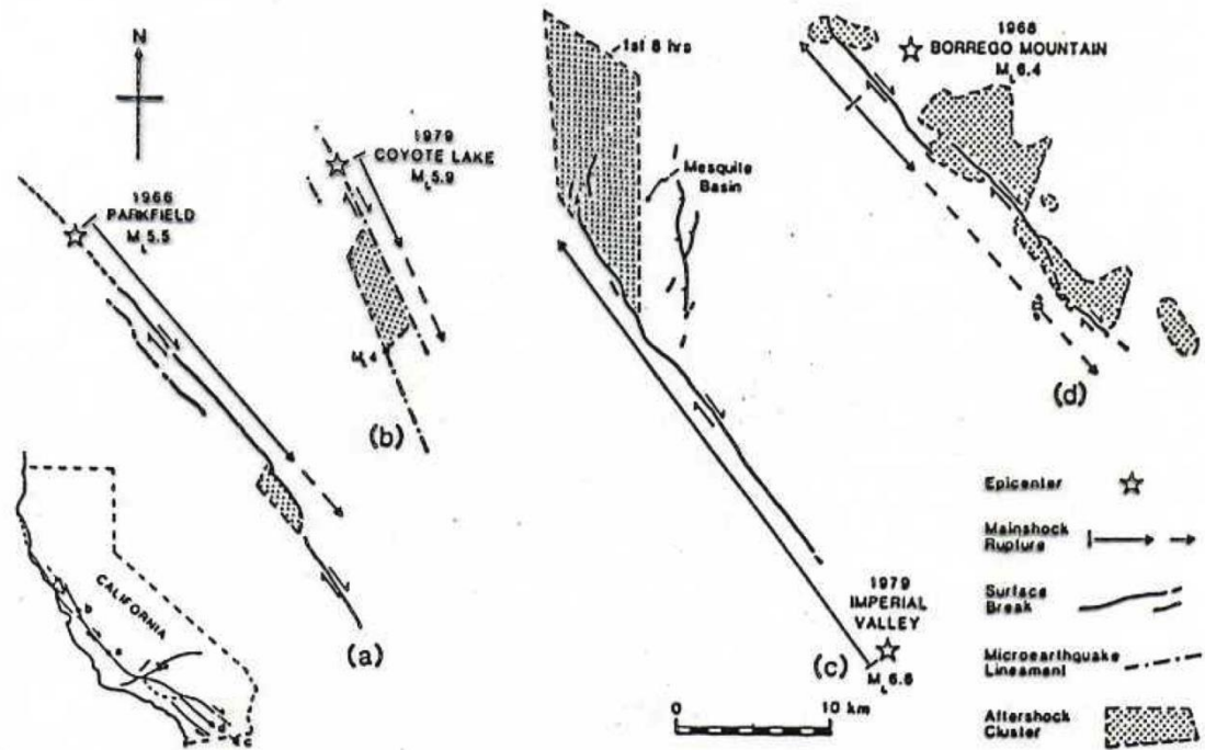
Fig. 3.33 Sketches showing ruptures terminated at jogs in the San Andreas fault zone: (a) Parkfield, 1966; (b) Coyote Lake, 1979; (c) Imperial Valley, 1979; (d) Borrego Mtn., 1968. (From Sibson, 1986c.)
