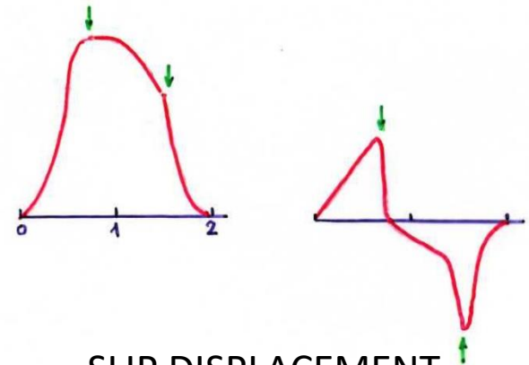
SLIP DISPLACEMENT AND VELOCITY OF P WAVES
